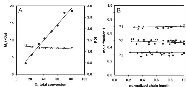
Figure 1. (A) Plot of M_n (●) and PDI (○) versus conversion for a batch copolymerization of 1 and 2 in THF at 0 °C ( [I] = [2] = 0.04 M; [Ni(dppp)Cl_2] = 0.002 M). (B) Plot of the cumulative mole fraction of 1 in the copolymer versus the normalized chain length for the batch copolymerizations ( 1 : 2 = 67:33 ( P1 , ▲); 50:50 ( P2 , ■); 33:67 ( P3 , ◆)).
